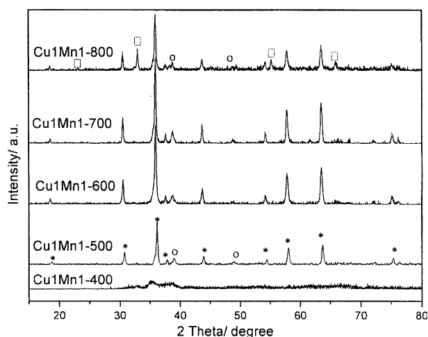
Figure 2. XRD patterns of Cu1Mn1-X catalysts. (□) \text{Mn}_2\text{O}_3 (*) \text{Cu}_{1.5}\text{Mn}_{1.5}\text{O}_4 (○) \text{CuO} .
