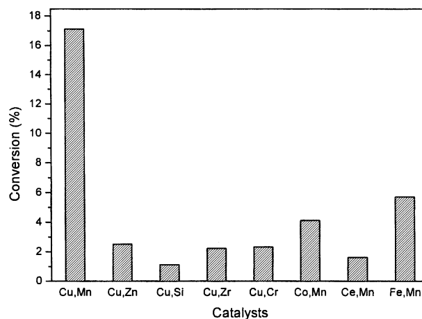
Figure 6. The conversions of toluene oxidation over hi-metallic oxides catalysts (Reaction conditions: 1.0 g catalysts, 50 ml toluene, 1.0 MPa O_2 , 2 h, 190 °C).
