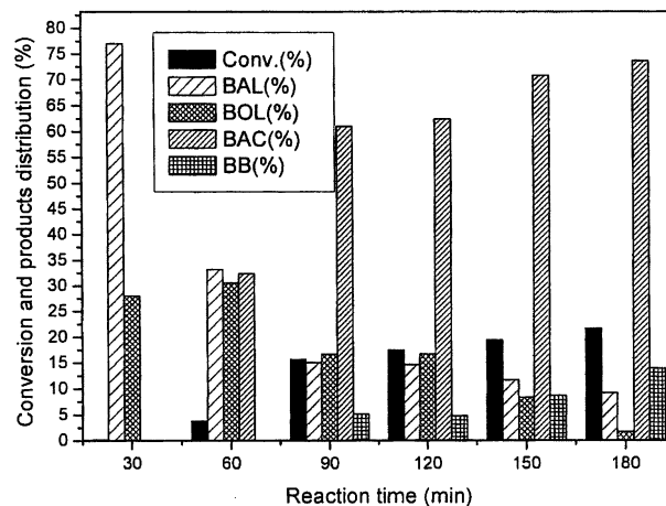
Figure 7. The product distributions at the different reaction time.
