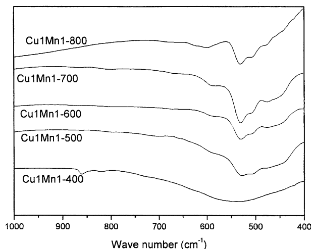
Figure 3. FT-IR spectra of Cu1Mn1-X.
