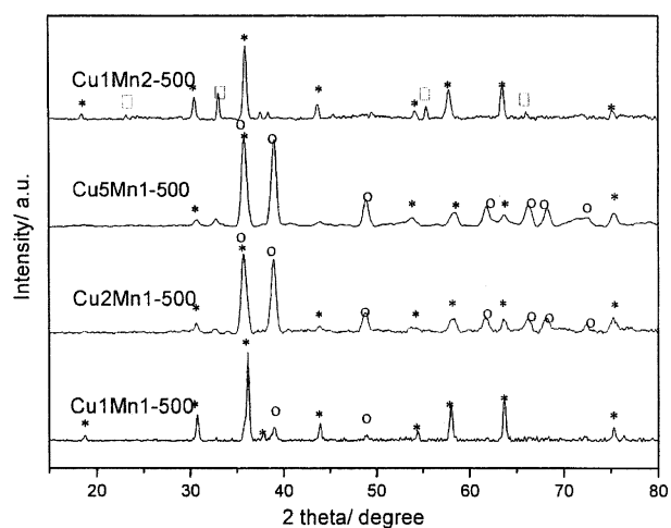
Figure 1. XRD patterns of CuAMnB-500, (*) \text{Cu}_{1.5}\text{Mn}_{1.5}\text{O}_4 , (○) CuO (□) \text{Mn}_2\text{O}_3 .
